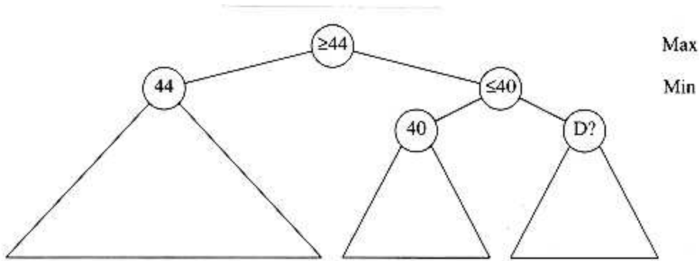
Figure 10.71 The node marked ? is unimportant
