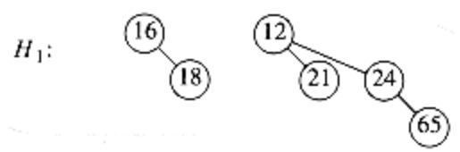
Figure 6.35 Binomial queue H_1 with six elements
