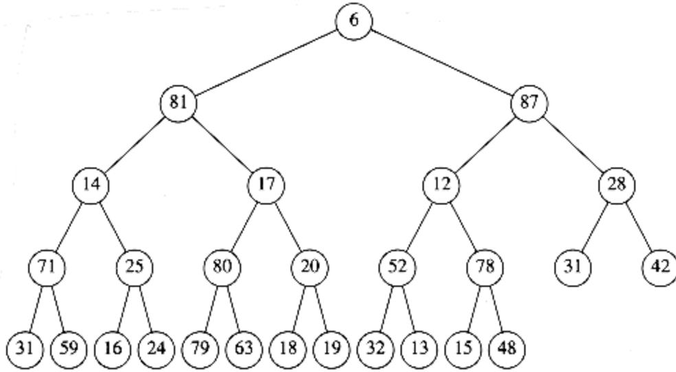
Figure 6.56 Min-max heap
