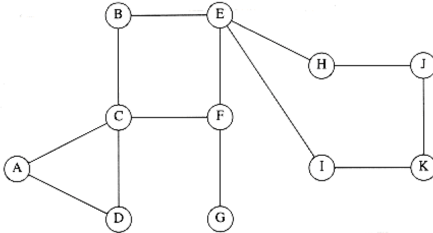
Figure 9.83
