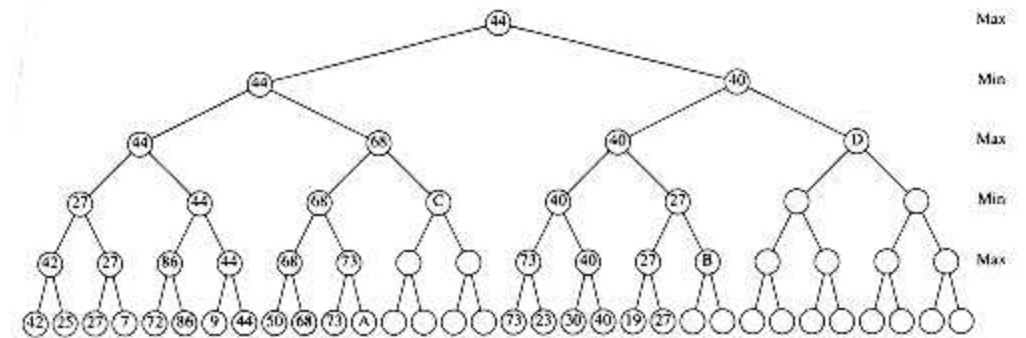
Figure 10.70 A pruned game tree
