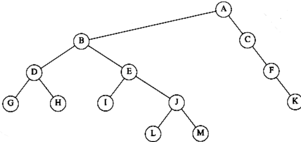
Figure 4.63
