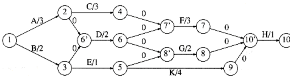
Figure 9.35 Event-node graph
