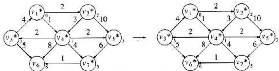
Figure 9.28 Stages of Dijkstra's algorithm
