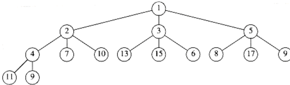
Figure 6.19 A d -heap
