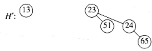
Figure 6.47 Binomial queue H', containing all the binomial trees in H3 except B3
