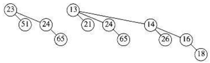
Figure 6.49 Result of delete_min(H3)
