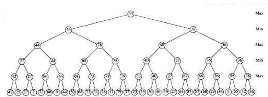
Figure 10.69 A hypothetical game tree
