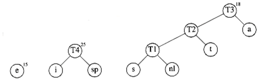
Figure 10.17 Huffman's algorithm after the fourth merge
