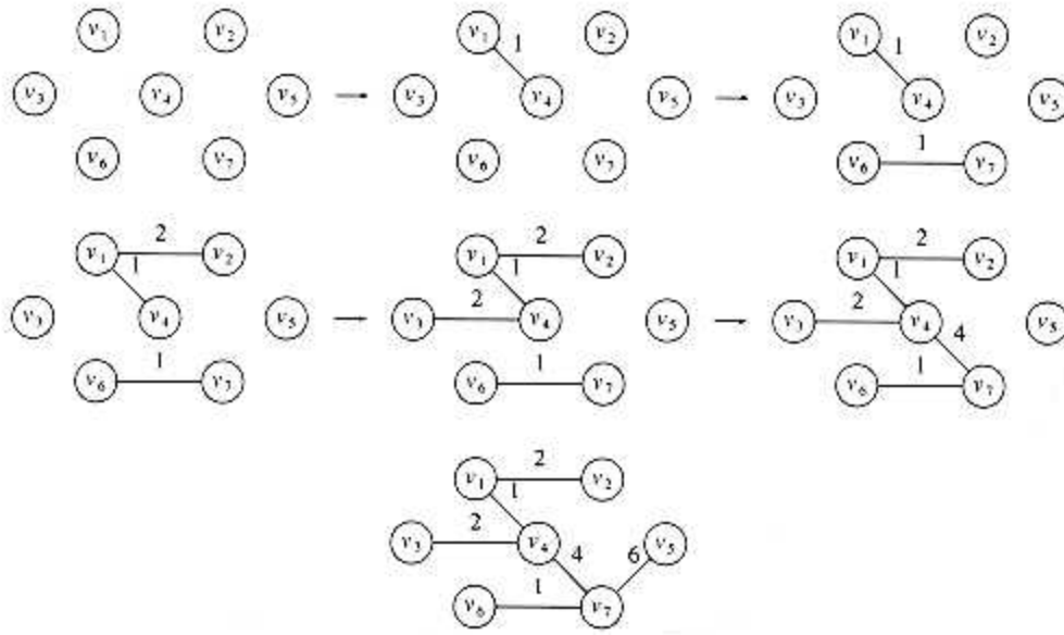
Figure 9.57 Kruskal's algorithm after each stage
