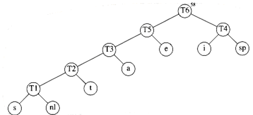
Figure 10.19 Huffman's algorithm after the final merge
