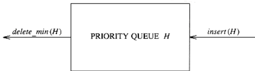
Figure 6.1 Basic model of a priority queue
