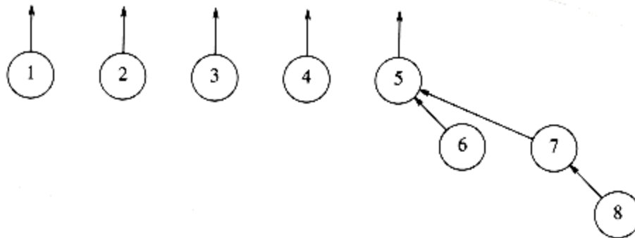
Figure 8.4 After union (5, 7)
