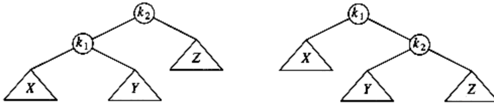
Figure 4.31 Single rotation
