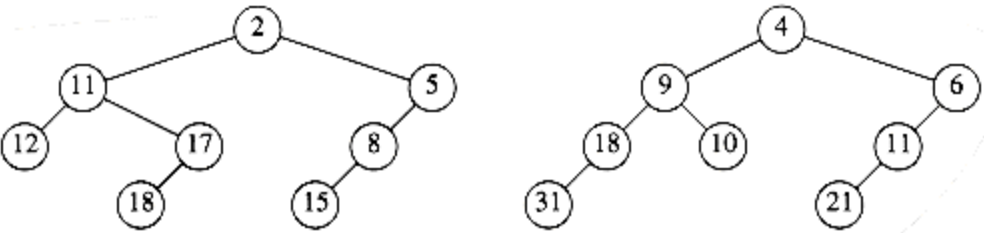
Figure 6.57
