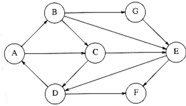
Figure 9.84
