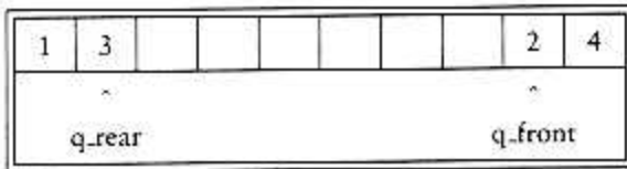
After Enqueue (3)
