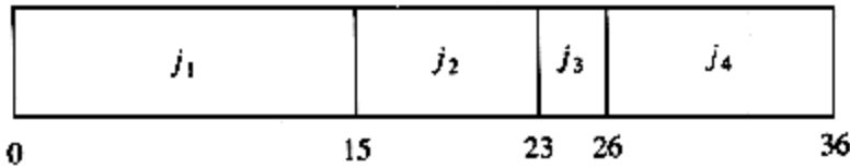
Figure 10.2 Schedule #1
