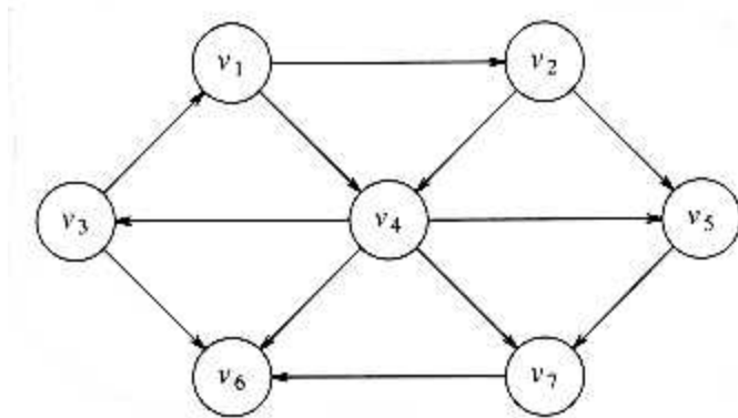
Figure 9.10 An unweighted directed graph G
