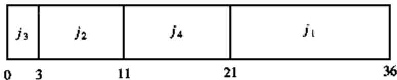
Figure 10.3 Schedule #2 (optimal)
