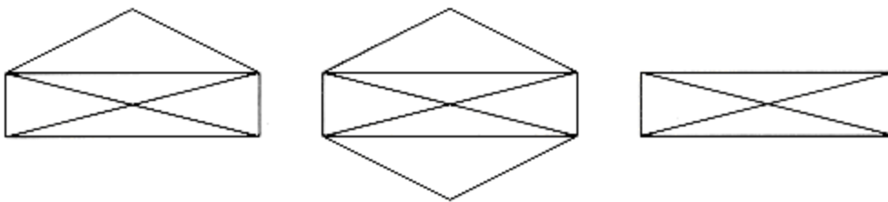
Figure 9.68 Three drawings
