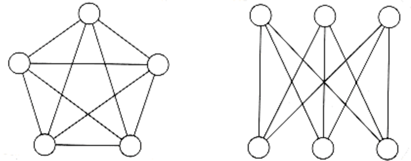
Figure 9.85
