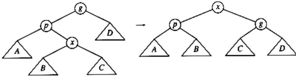
Figure 4.42 Zig-zag
