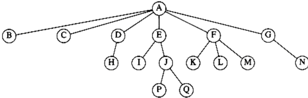
Figure 4.2 A tree
