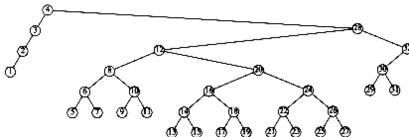
Figure 4.47 Result of splaying previous tree at node 3
