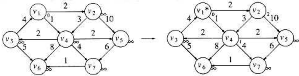
Figure 9.27 After v_6 is declared known and algorithm terminates
